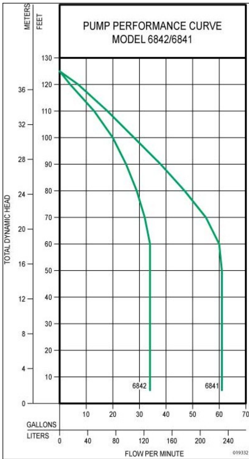
6841/6842 PERFORMANCE DATA
